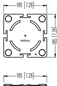
Base Connector
